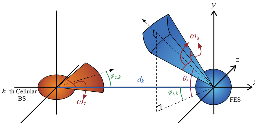
FIGURE 1 System model on the ground where the cellular BSs and the FES exist.
