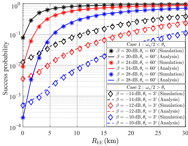
FIGURE 5 Success probability of FES for various exclusion zone radius values, R_{EE}
